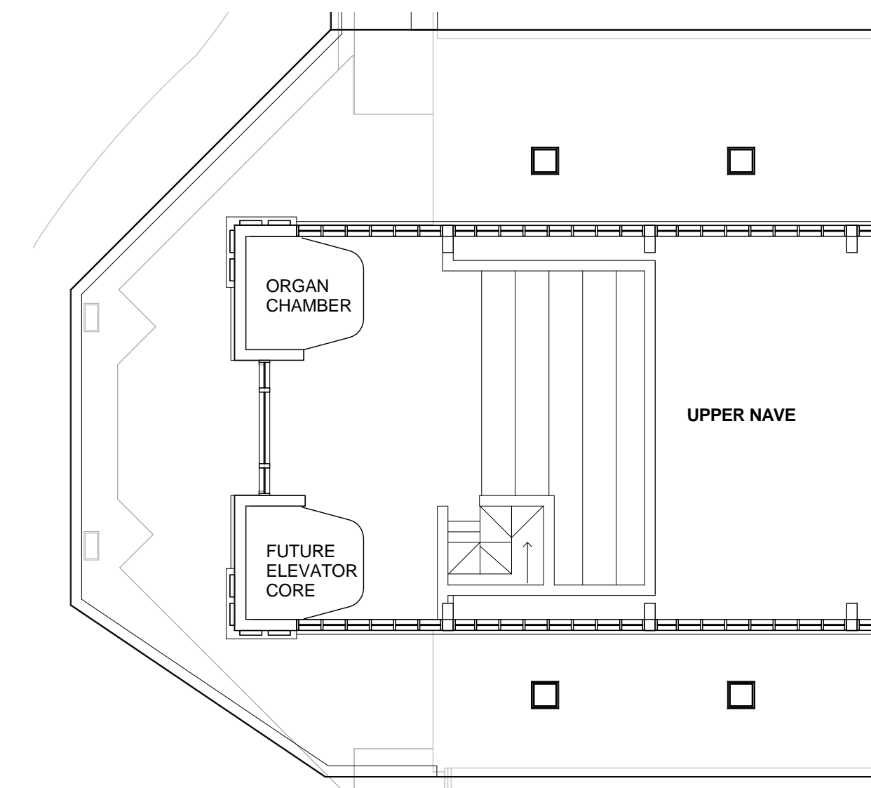
CHURCH BALCONY PLAN PHASE 1 3/32" = 1'-0"
