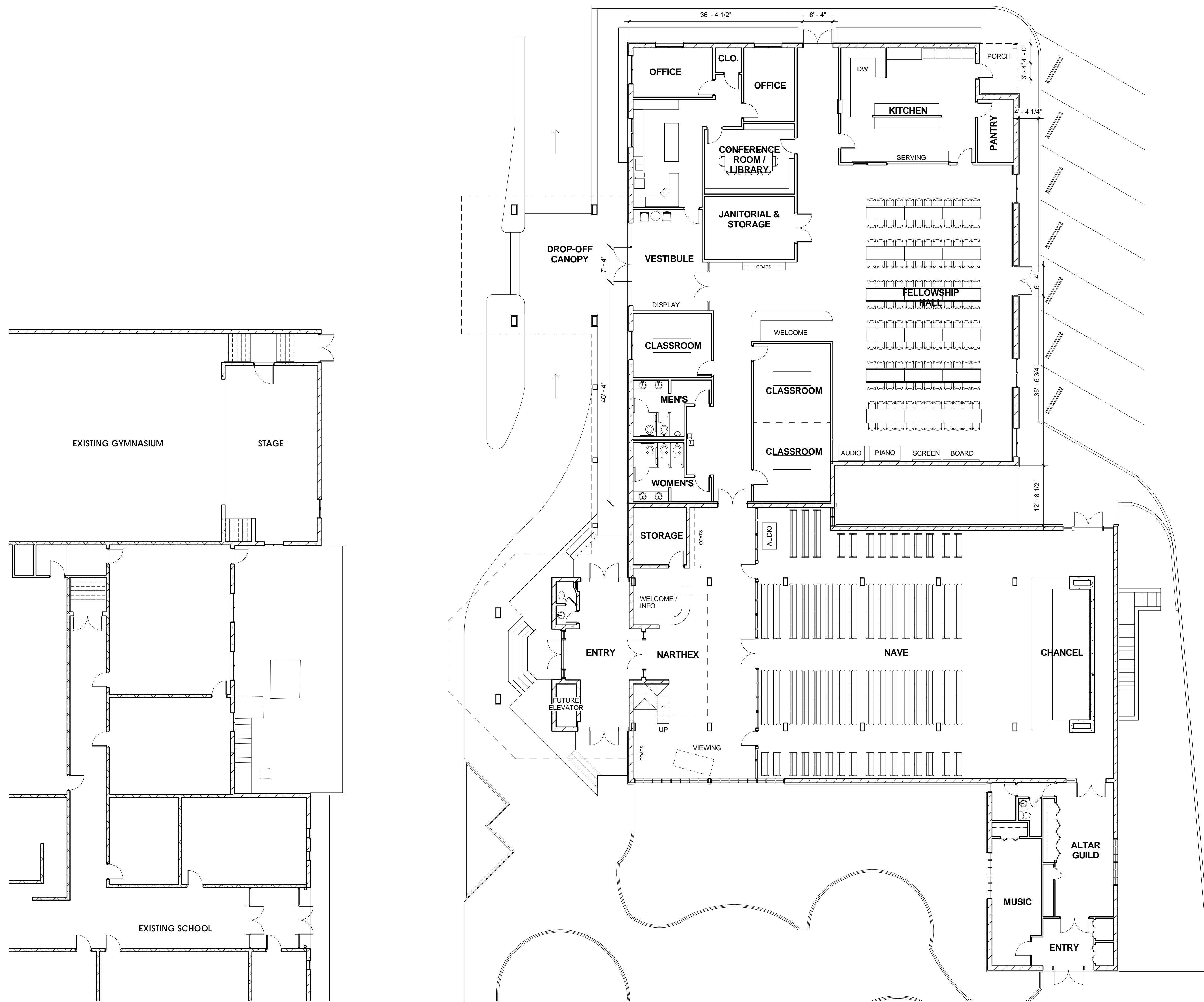
FLOOR PLAN PHASE No.1 3/32" = 1'-0"
